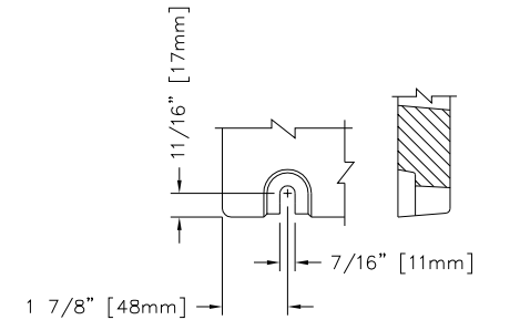
TYPICAL BOLT SLOT DETAIL SCALE 1:4
